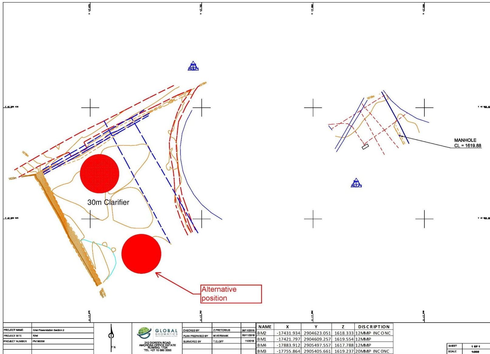
Figure 3: Proposed location of the clarifier on the southern section of the Cooling Towers at the Kriel Power Station.
